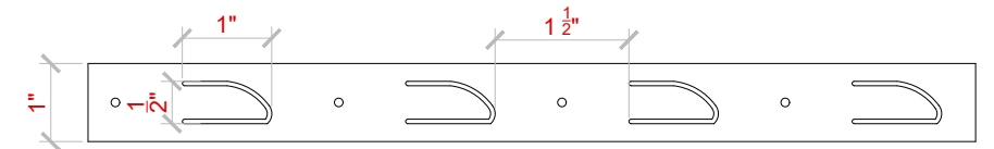
L MOLDING
