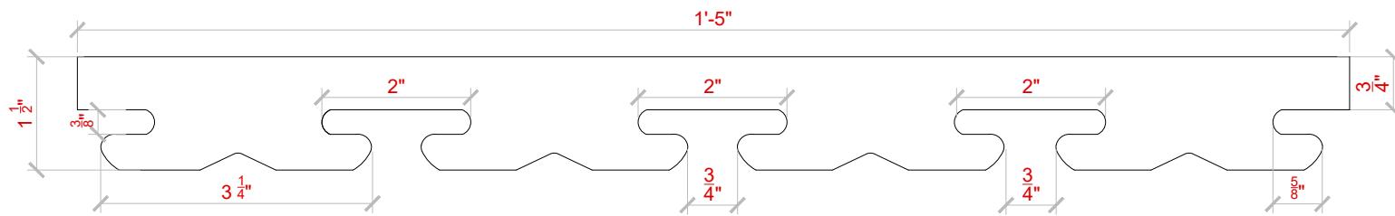
CARRIER
